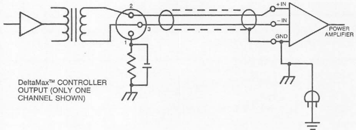
FIGURE 7 - DeltaMax™ Output Connection
