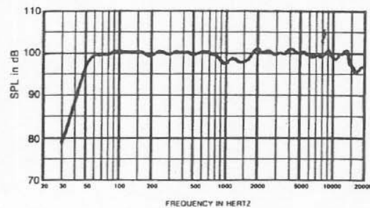
FIGURE 2 - DMC-1152B/DML-1152A Axial Frequency Response (1 watt/1 meter into LF midband)
