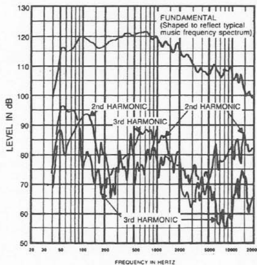
FIGURE 6 - DMC-1152B/DML-1152A Harmonic Distortion (120 dB SPL/1 meter using typical music frequency spectrum)
