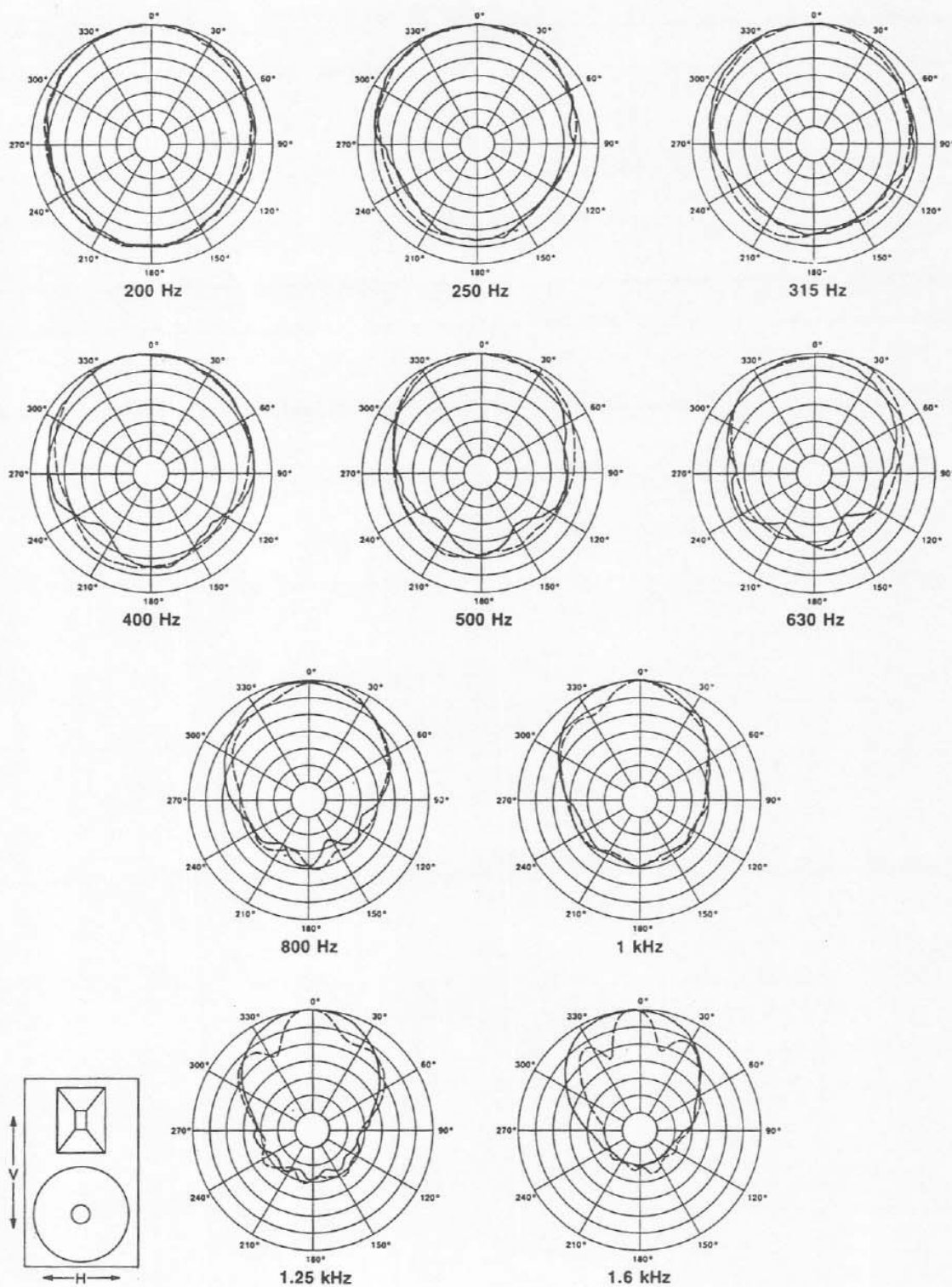
FIGURE 3 - DMC-1152B/DML-1152A Polar Response (1/3-octave pink noise, 4 volts at 20 feet)
