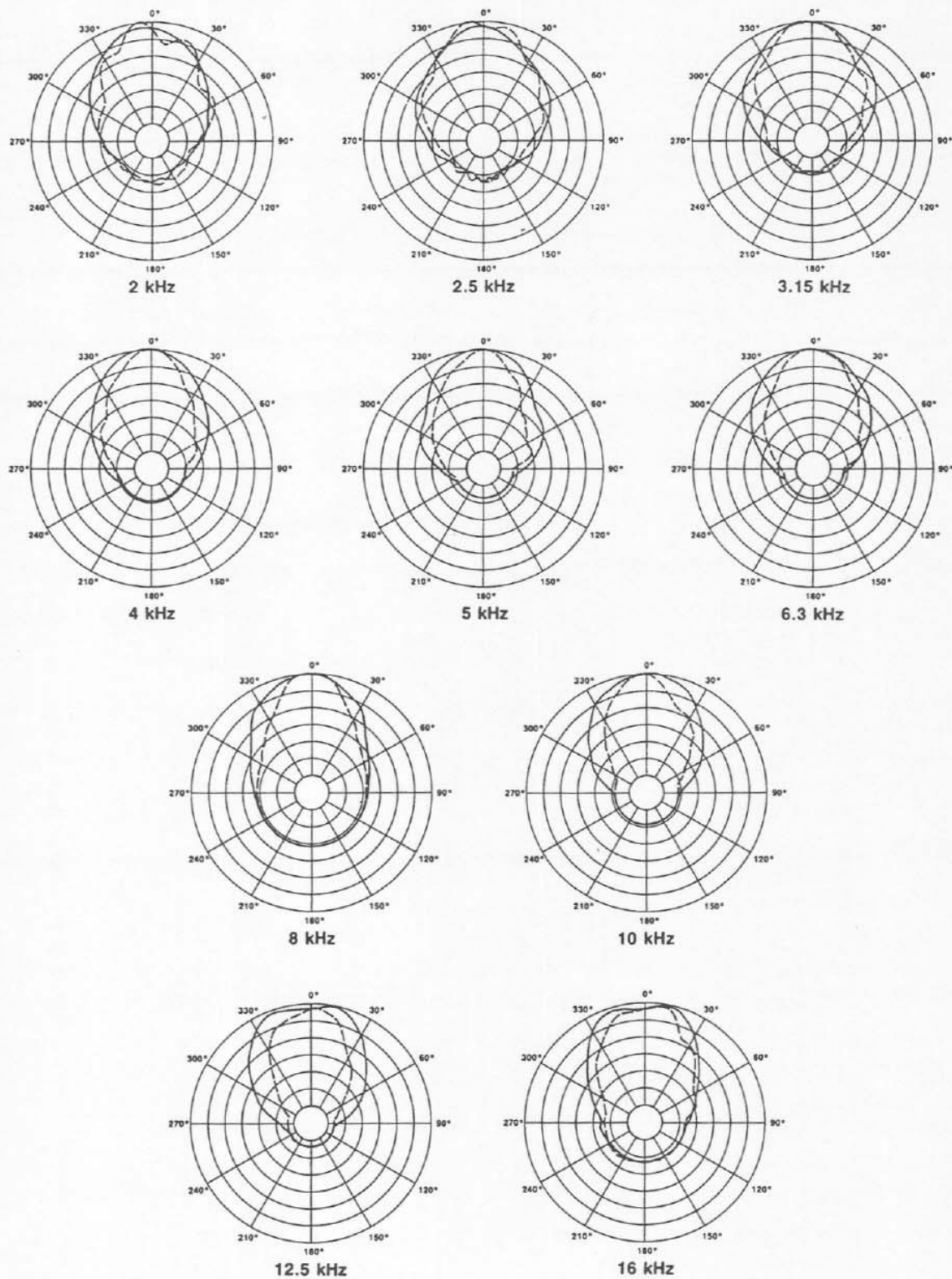
FIGURE 3 (continued) - DMC-1152B/DML-1152A Polar Response ( 1/3 -octave pink noise, 4 volts at 20 feet)
