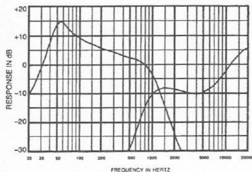
FIGURE 1 - DMC-1152B Frequency Response
